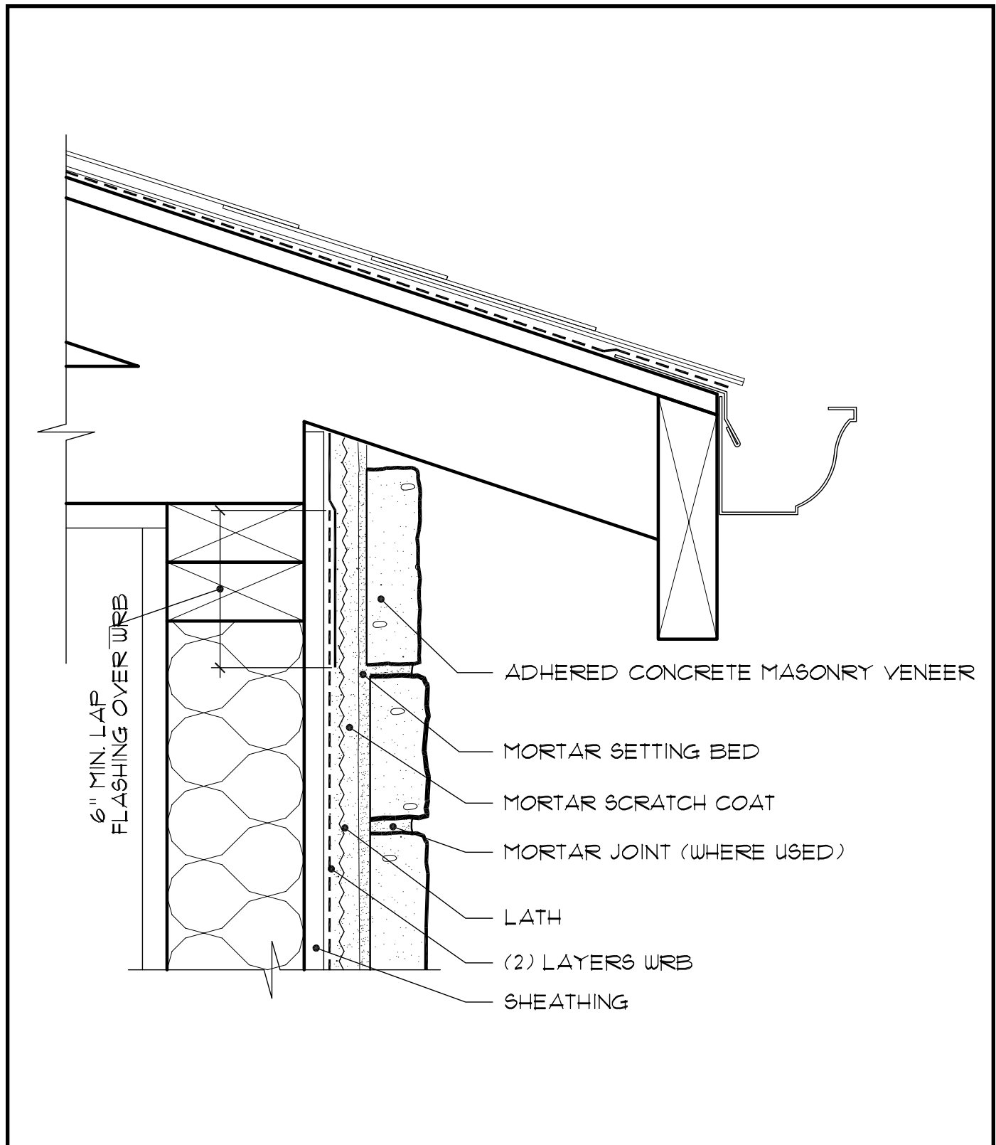
Fig. 11. Open Eave - Overhang
