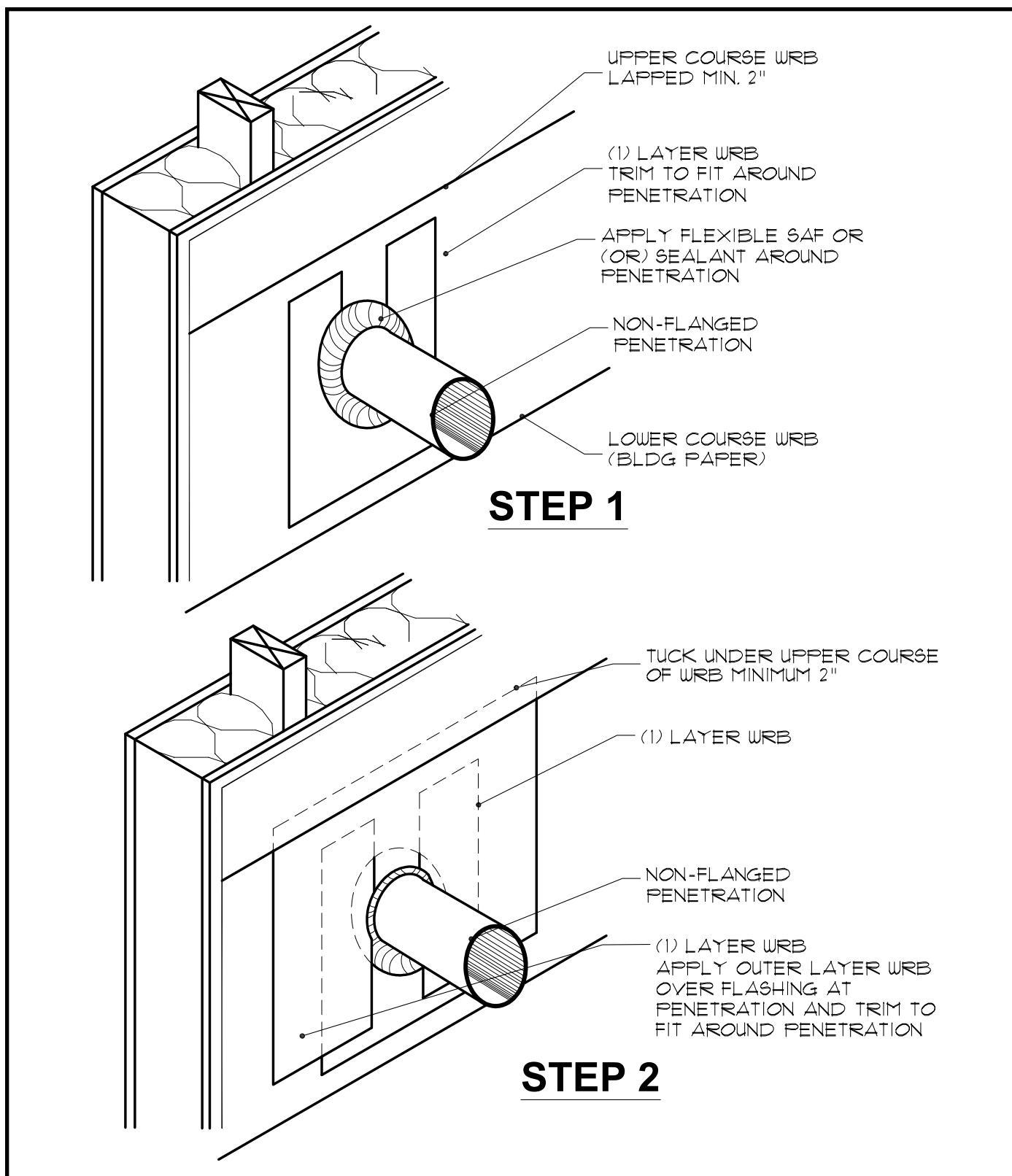
Fig. 28. Penetration Non-Flanged, with Building Paper WRB
