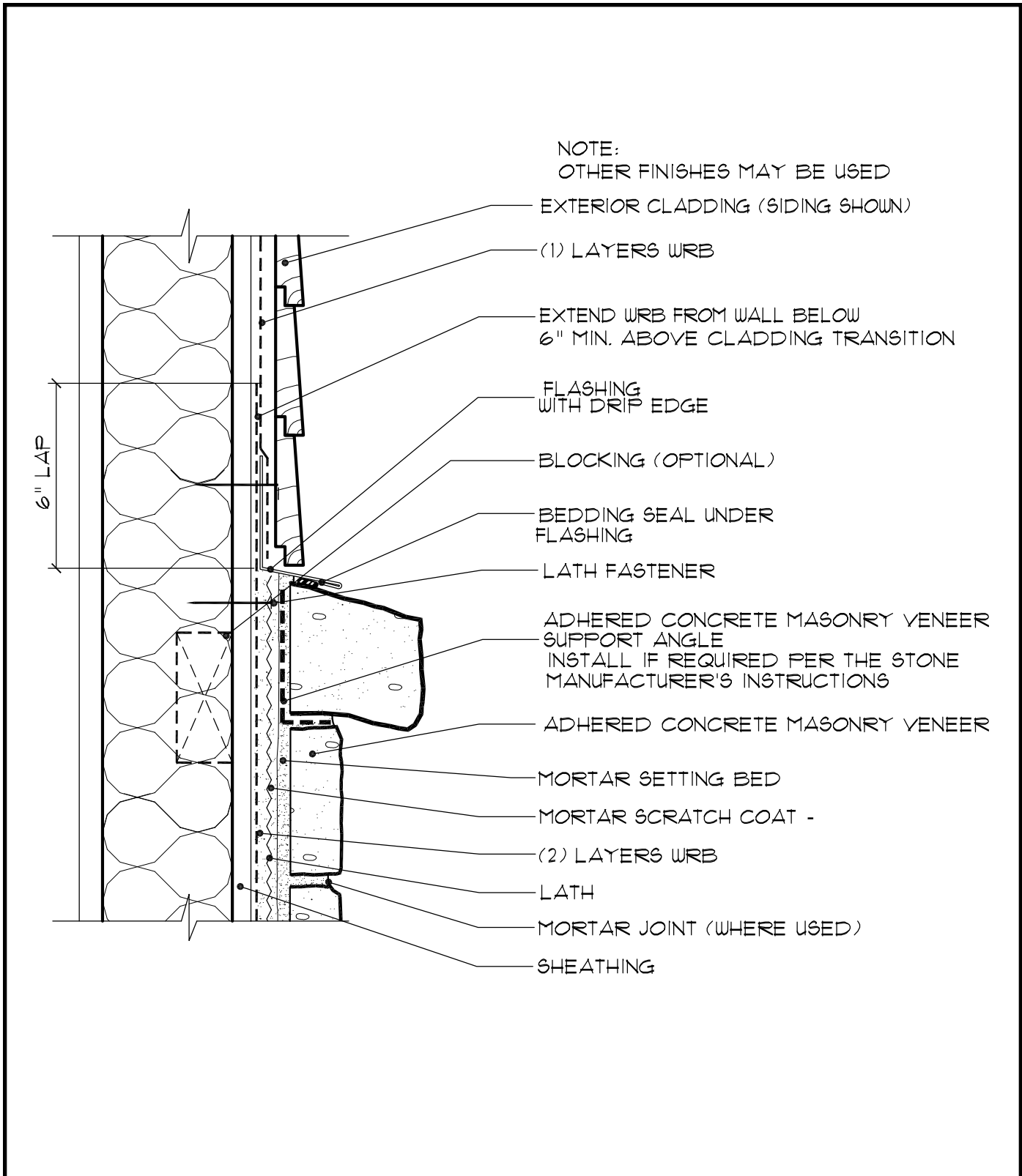
Fig. 6. Cladding Transition
