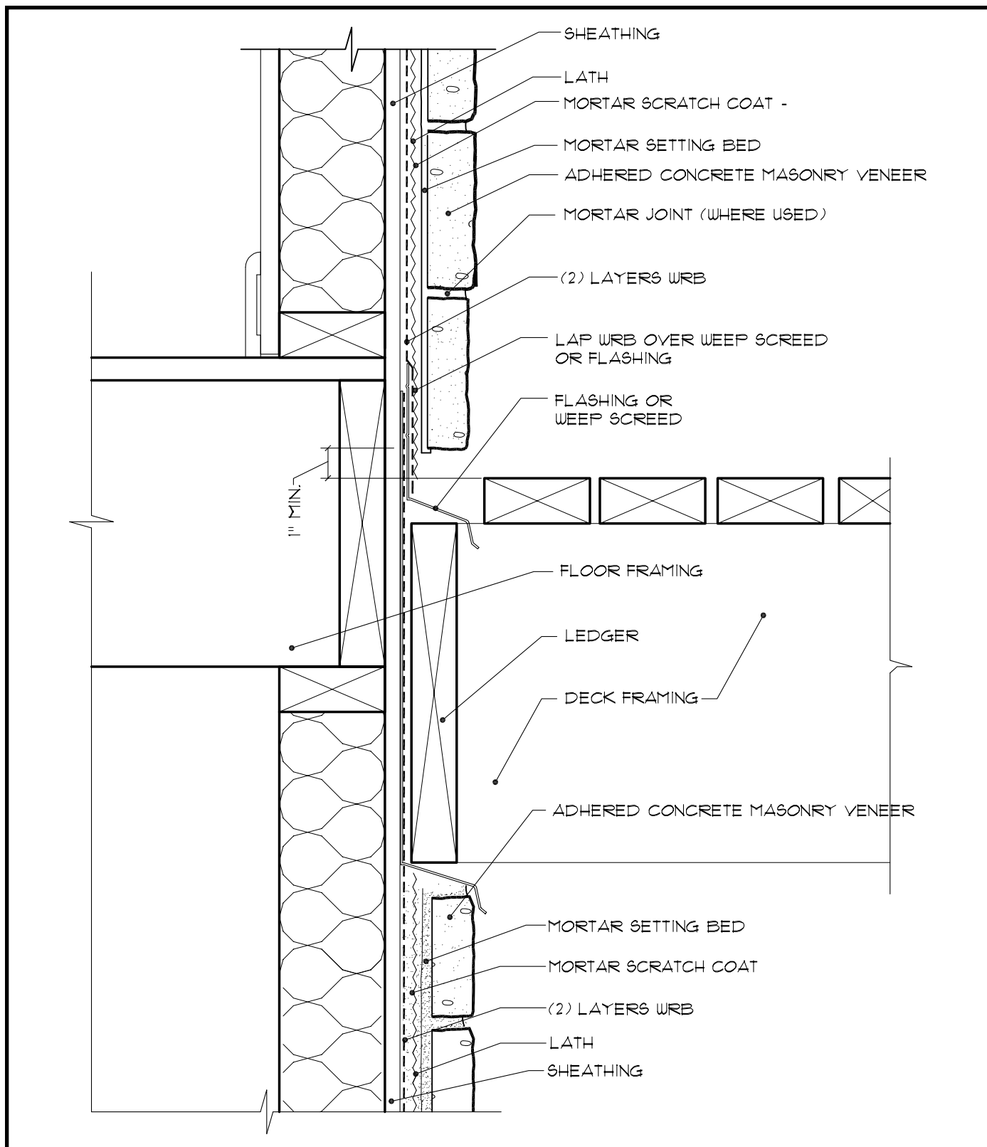
Fig. 32. Deck Termination
