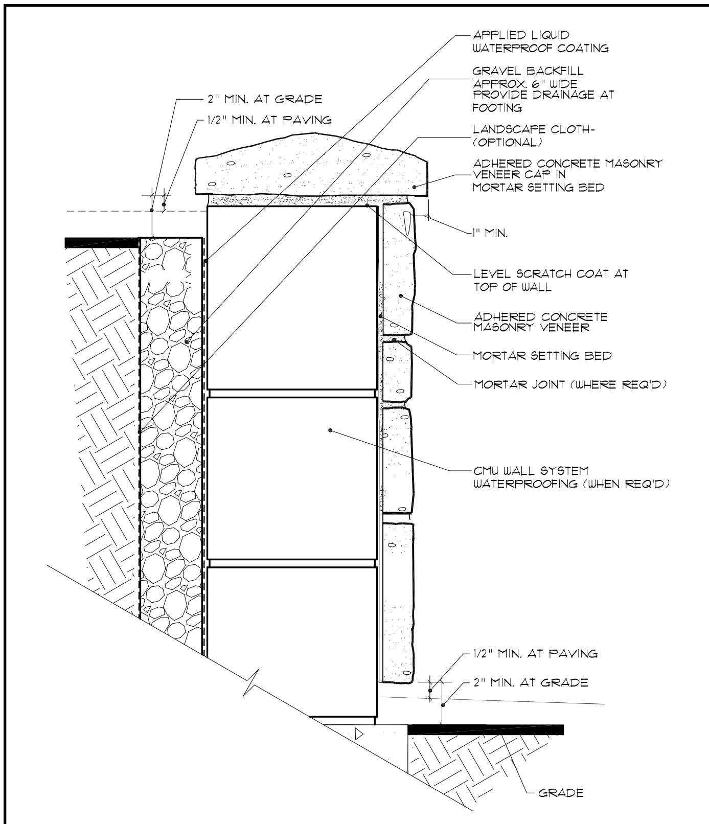
Fig. 38. Retaining Wall (CMU)
