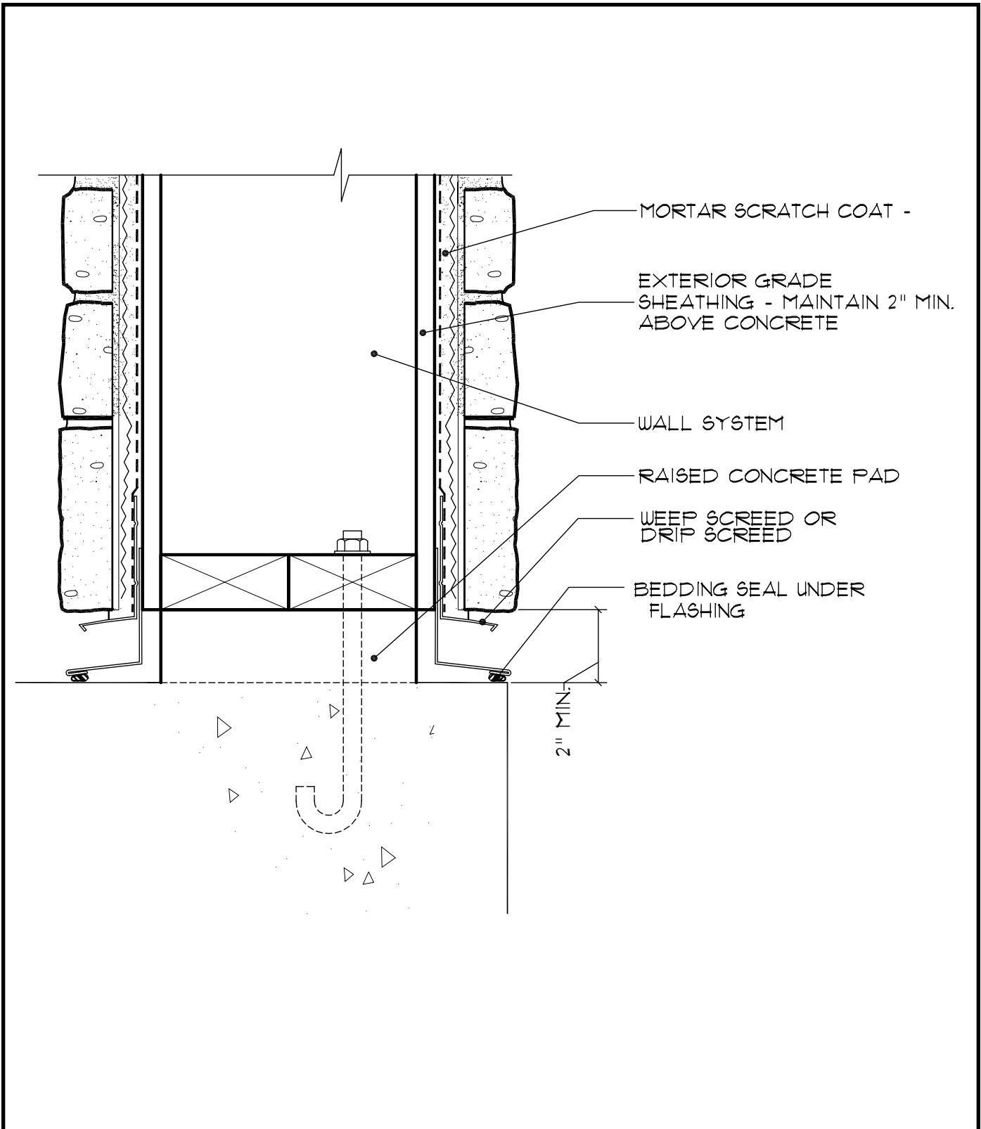
Fig. 26. Raised Column Base
