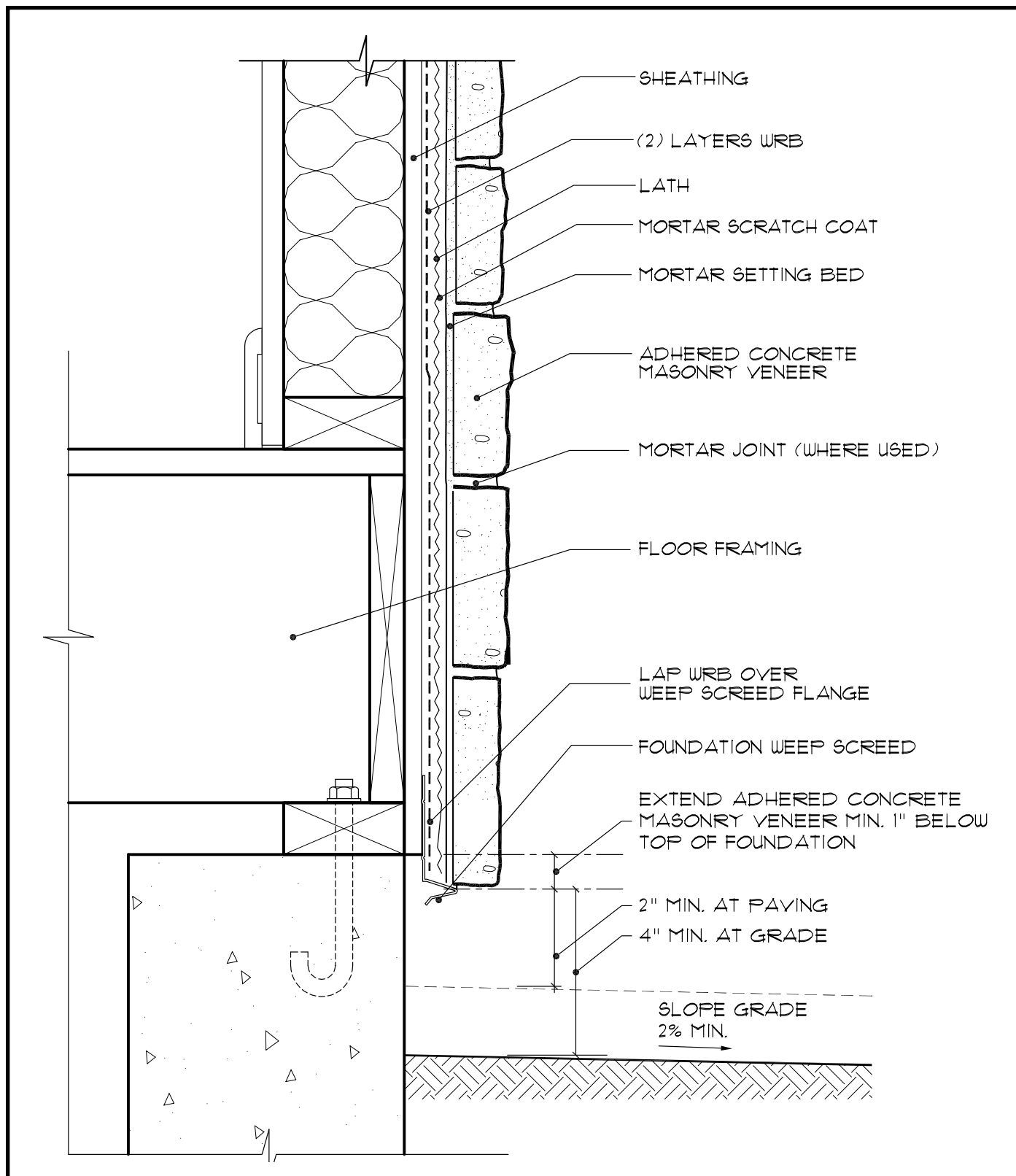
Fig. 3. Foundation Wall Base
