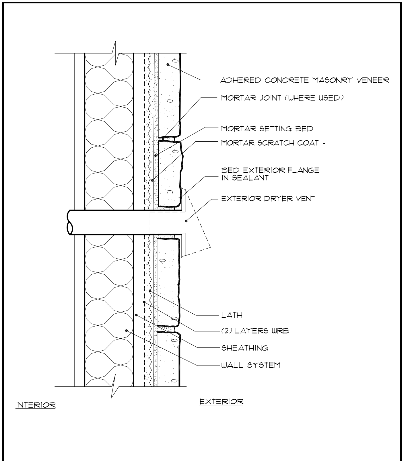
Fig. 31. Penetration, Dryer Vent
