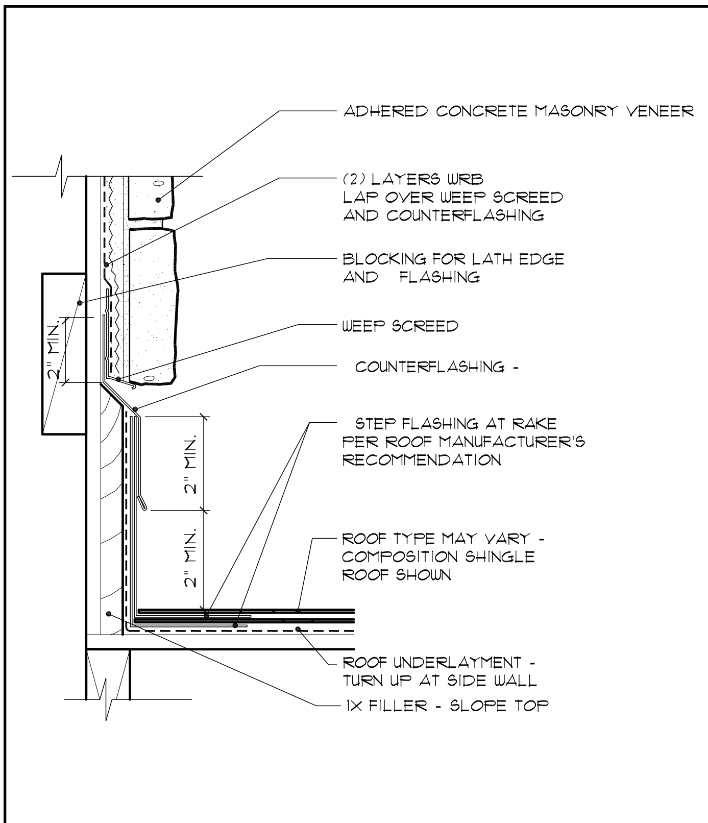
Fig. 16. Side Wall - Composition Shingles Curbing
