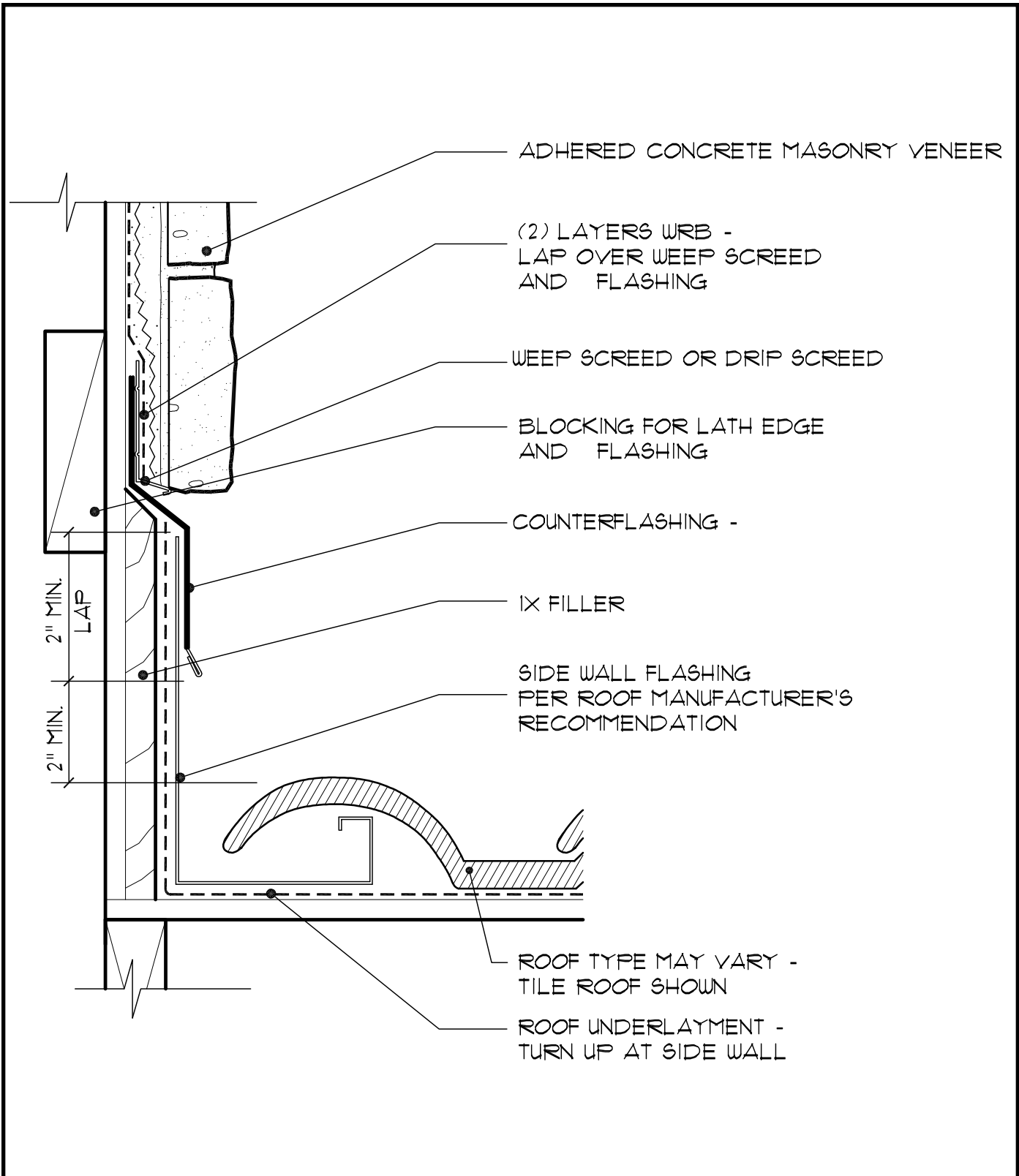
Fig. 18. Side Wall - Tile Roofing Curbing
