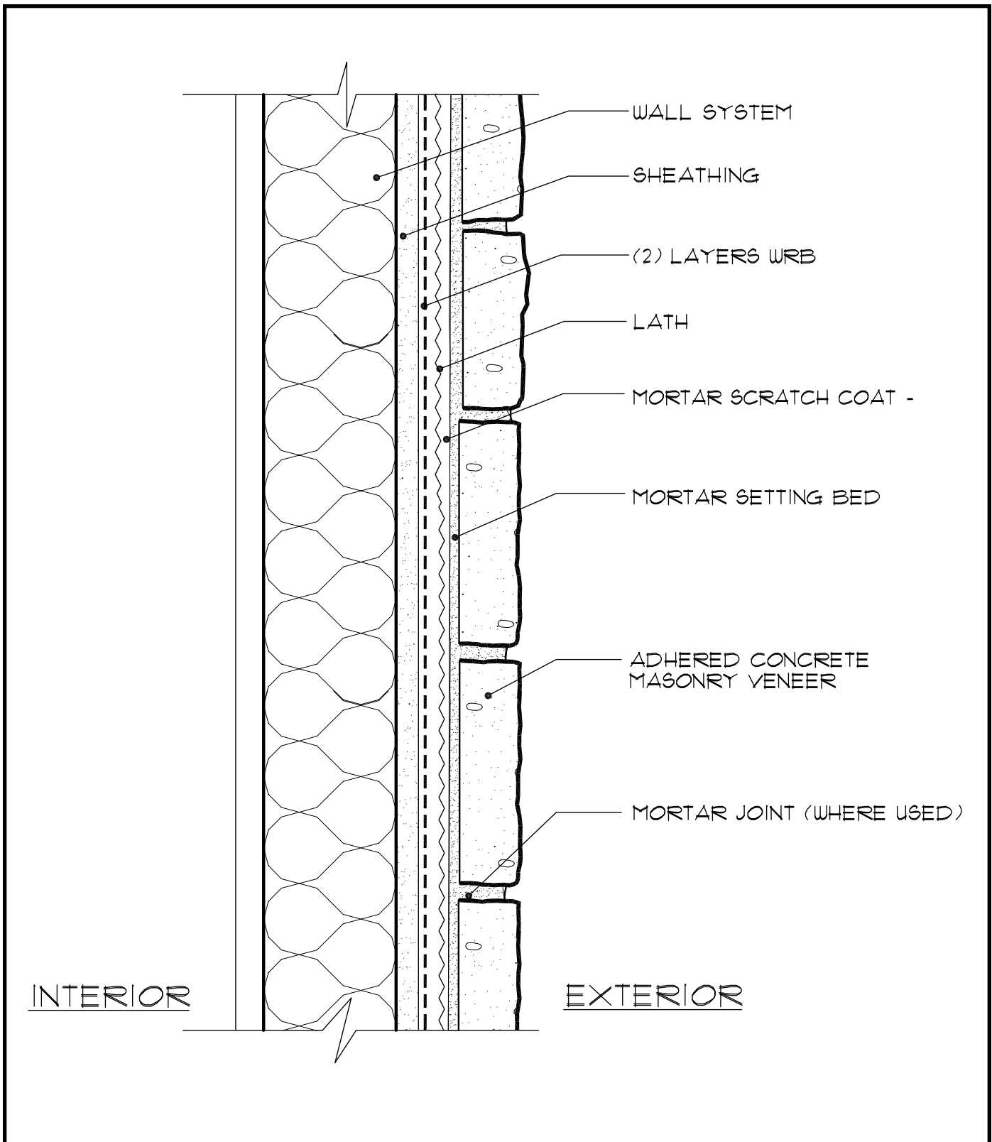
Fig. 2. Typical Wall Section
