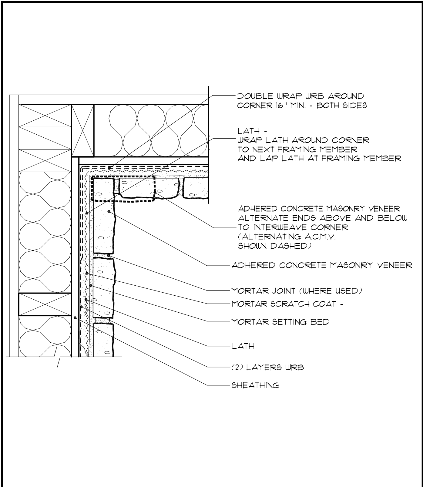
Fig. 8. Inside Corner
