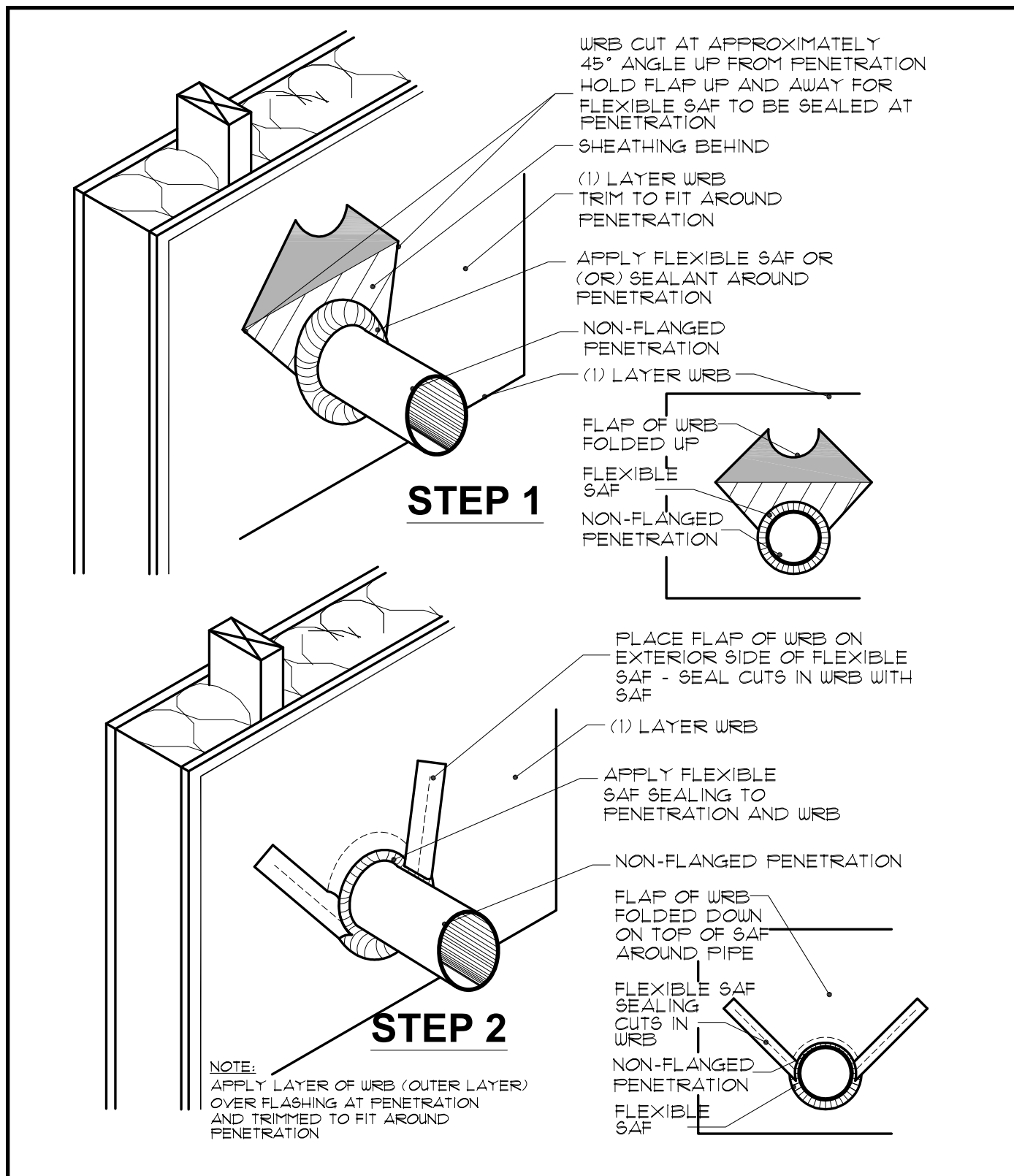
Fig. 29. Penetration Non-Flanged, with Housewrap WRB
