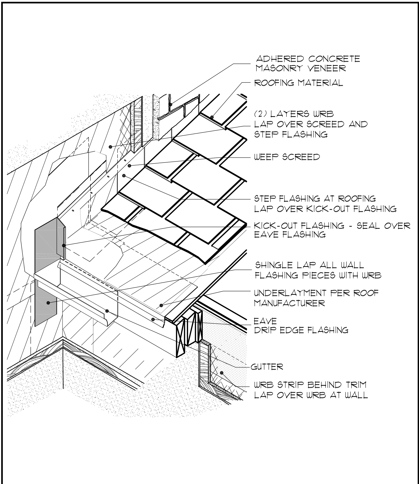
Fig. 22. Kick-Out Flashing
