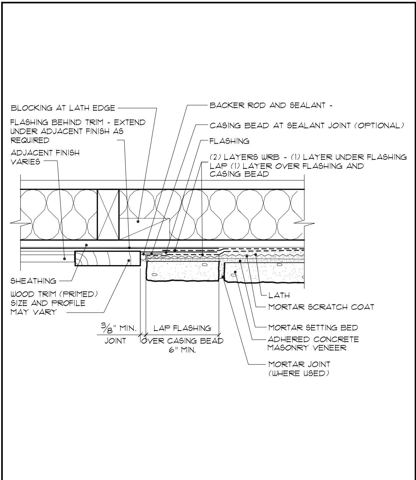
Fig. 10. Vertical Transition
