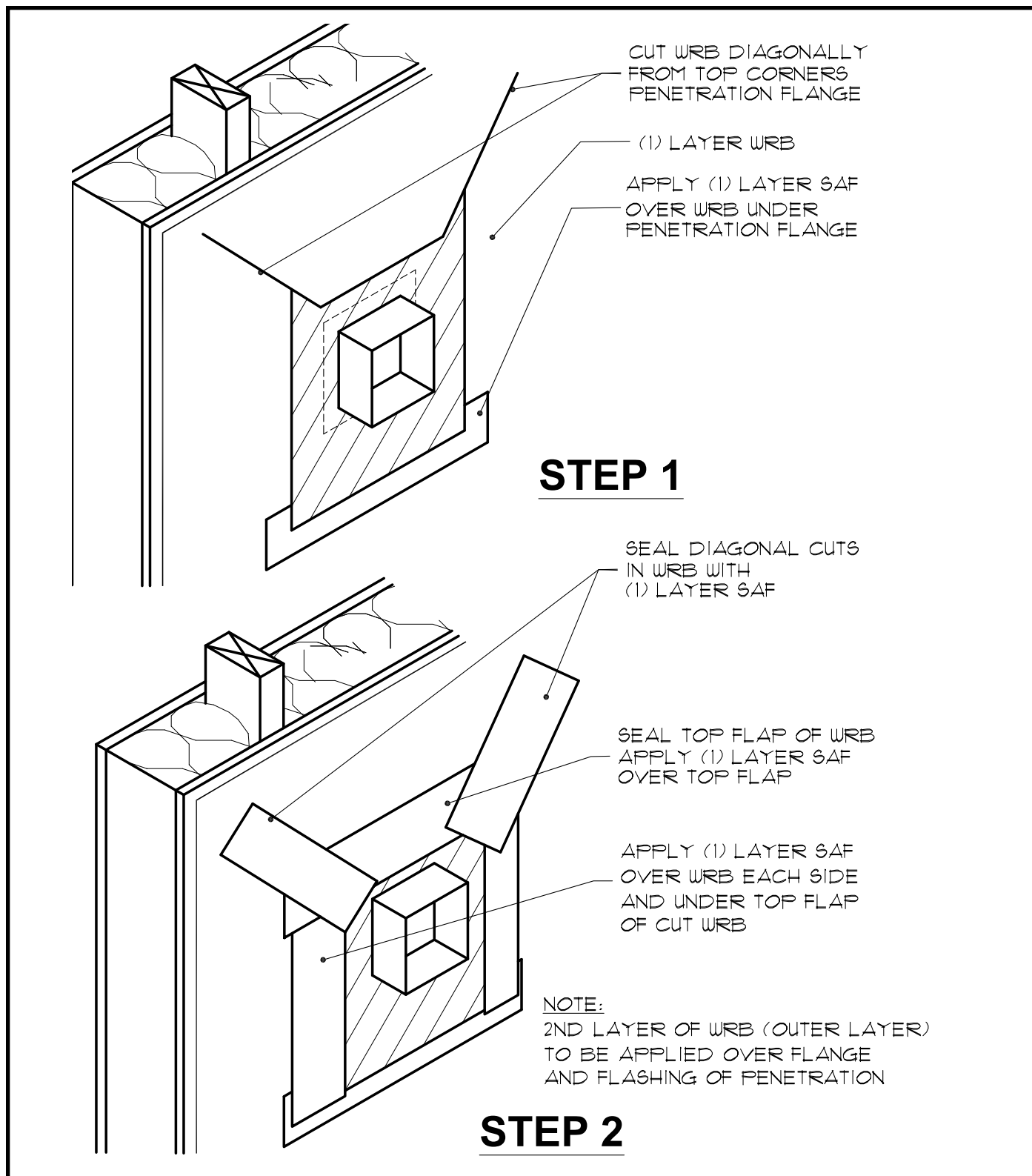
Fig. 27. Penetration, Flanged
